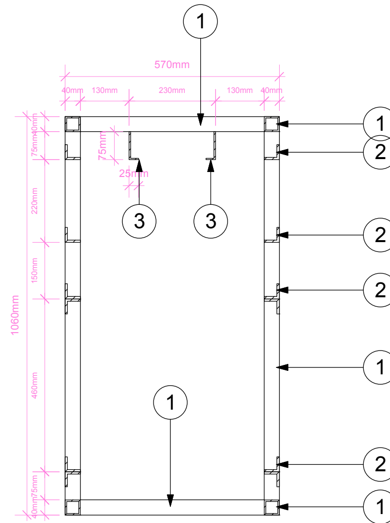
ISLAND BASIN STAINLESS STEEL FRAME SECTION AA
